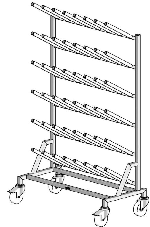
DIMETRIC VIEW
