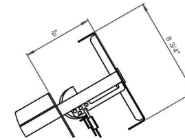
DETAIL K SCALE (1 : 4) TOP TIER LOCK PLATE OPEN
