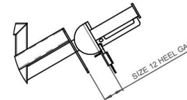
DETAIL M SCALE (1 : 4) TOP TIER LOCK PLATE CLOSED (UK 12 POSITION)
